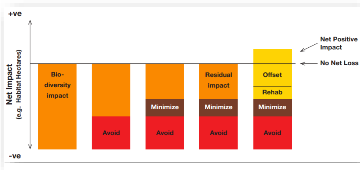
Figure 7: Mitigation Hierarchy
